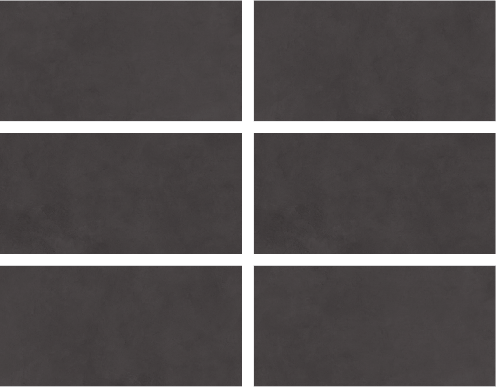
Random - 3 Faces
